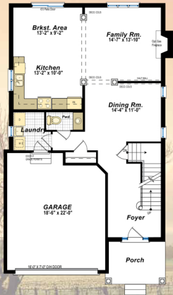
Ground Floor 1,046 Sq.Ft.
