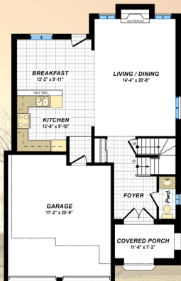
Ground Floor 869 Sq.Ft.
