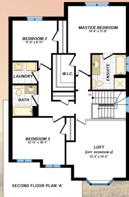
Second Floor 1,152 Sq.Ft.
